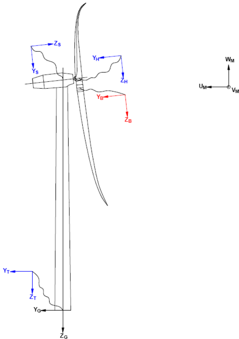
Figure 1. Illustration of coordinate system as result of user input from example in section Example of main input file at page 93. There are two coordinate systems in black which are the default coordinate systems of global reference and default wind direction. The blue coordinate systems are main body coordinate systems attached to node 1 of the substructure, the orientation of these are fully determined by the user. The red coordinate systems are also defined by the user, but in order to make the linkage between aerodynamic forces and structure work these have to have the z from root to tip, x in chordwise direction and y towards the suction side.
