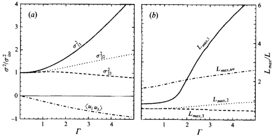
Figure 4: Turbulence characteristics compared to isotropic conditions as function of gamma parameter, Mann.. Left: Relation between variance is changed for higher shear distortions. Right: The relation between length scales are also changed for non-isotropic turbulence. It is recommended to use \Gamma = 3.9 for normal atmospheric conditions. This is also the requirement in the IEC61400-1 standard. Isotropic conditions are obtained using \Gamma = 0 .
